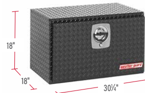
▼ Model 631-5-02
