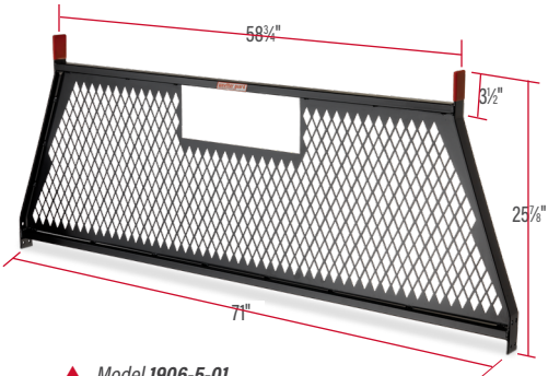
▲ Model 1906-5-01
